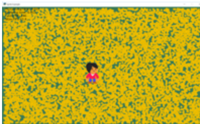
Fig. 122: stress_test_collision
