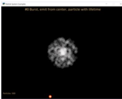
Fig. 114: particle_systems
