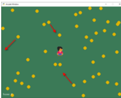
Fig. 26: sprite_collect_coins_move_bouncing
