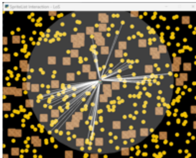
Fig. 103: spritelist_interaction_visualize_dist_los
