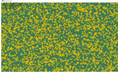
Fig. 121: stress_test_draw_moving
