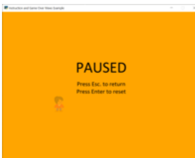
Fig. 63: view_pause_screen
